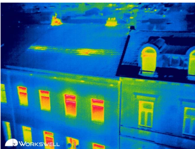
Construction roof thermal bridges. They may be signs of serious roof damage and leaks.
