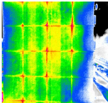
Thermal bridges.
